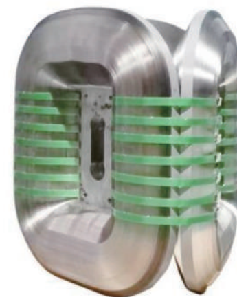
Real picture of an amorphous three-dimensional wound core
